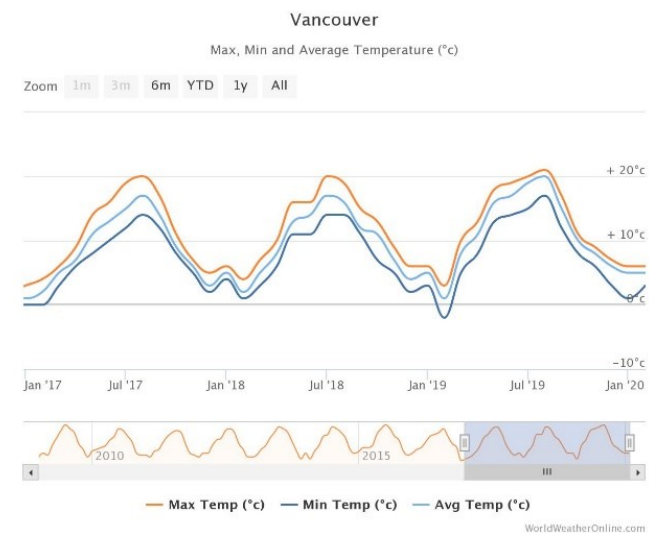
Supplementary Figure 1. Three and ten year temperature data (through February 2020) from seven cities currently affected and five at potential risk of epidemic spread. In the months that cities had outbreaks of COVID-19, minimum and average temperature was > 0^{\circ}\text{C} , and outbreaks occurred during prolonged temperature nadirs that typically lasted > 1 month. Temperature graphs for five cities potentially at risk also provided (Beijing, Prague, Glasgow, Manchester, and Vancouver,).
